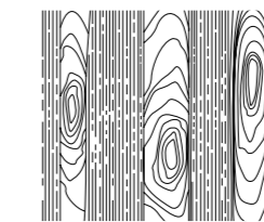
Brettcharakter | Mismatch
